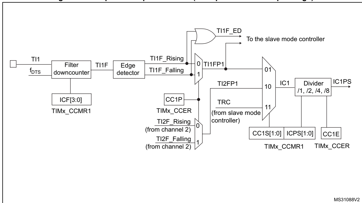
Figure 178. Capture/compare channel (example: channel 1 input stage)
