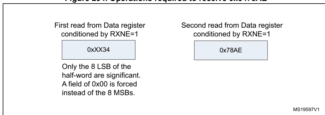
Figure 294. Operations required to receive 0x3478AE
