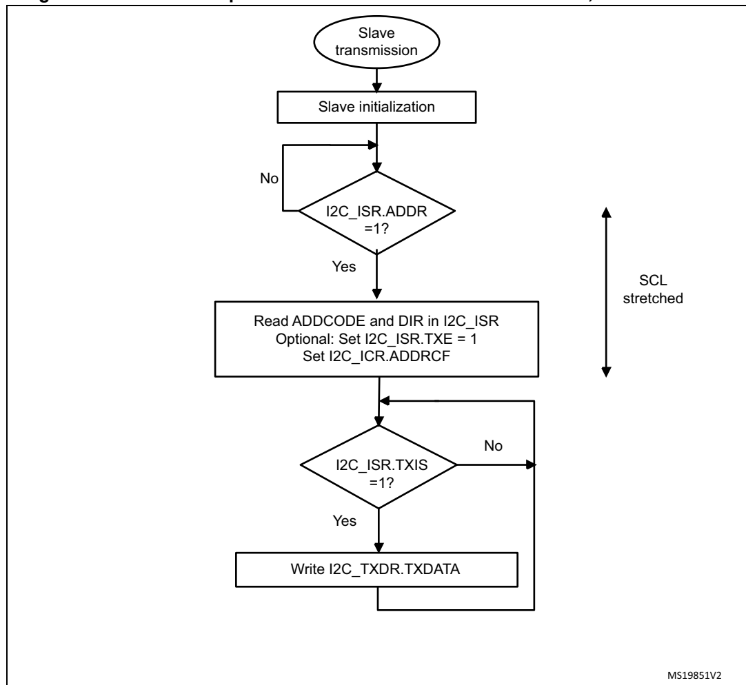
Figure 217. Transfer sequence flowchart for I2C slave transmitter, NOSTRETCH=0
