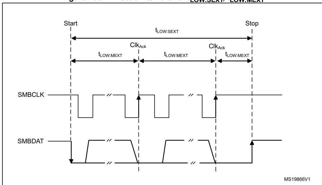
Figure 233. Timeout intervals for t_{\text{LOW:SEXT}} , t_{\text{LOW:MEXT}}
