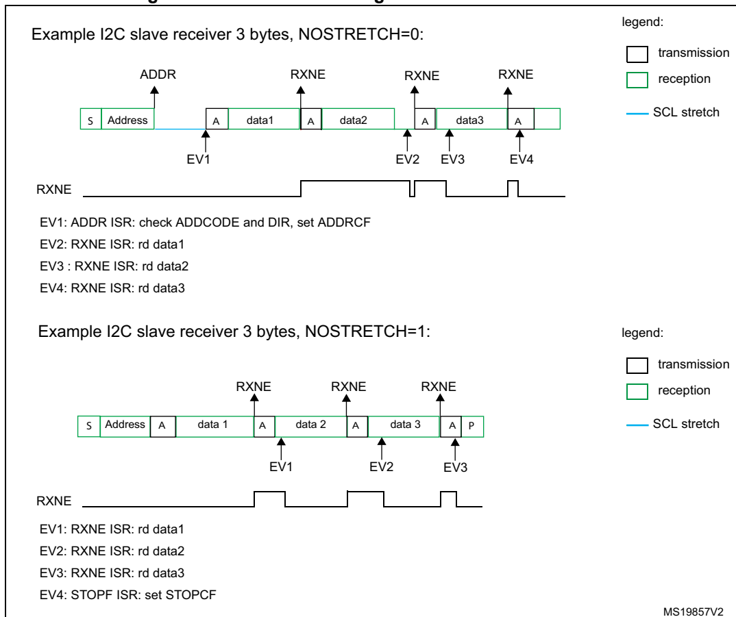
Figure 222. Transfer bus diagrams for I2C slave receiver
