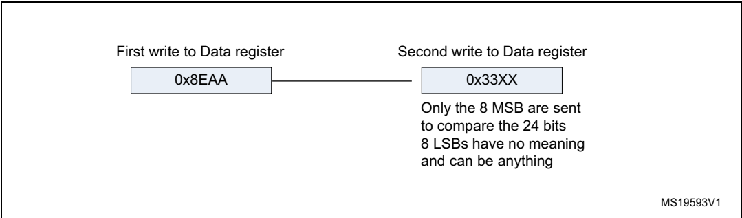
Figure 284. Transmitting 0x8EAA33
