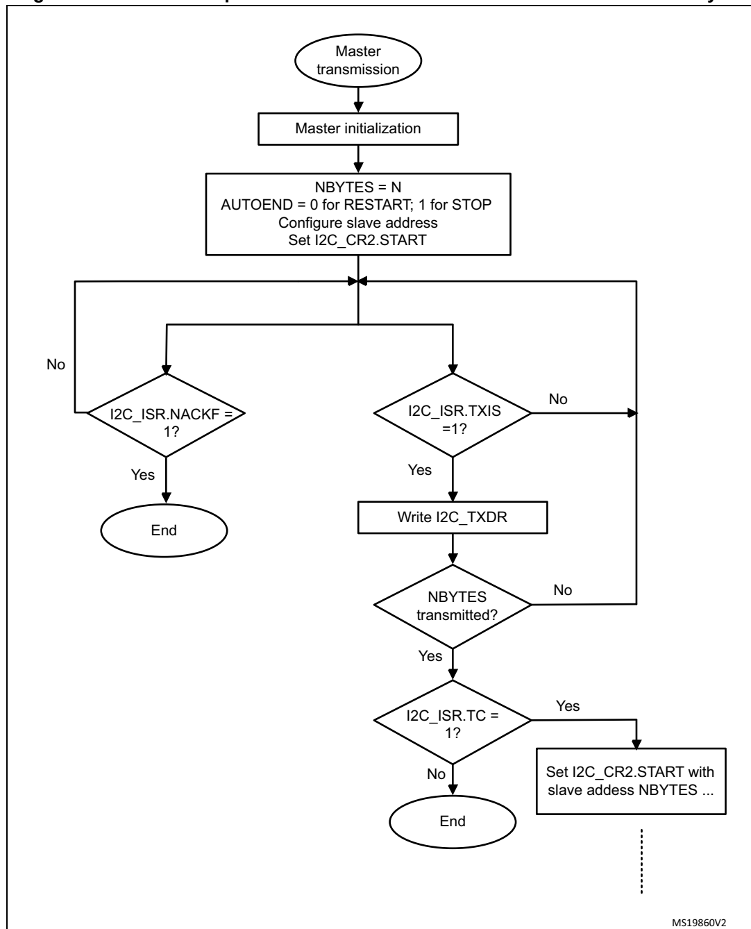
Figure 227. Transfer sequence flowchart for I2C master transmitter for N \leq 255 bytes
