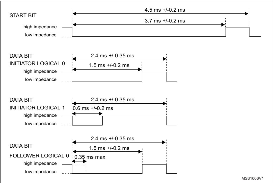
Figure 327. Bit timings
