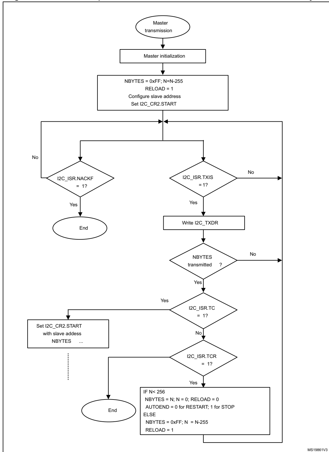
Figure 228. Transfer sequence flowchart for I2C master transmitter for N&gt;255 bytes
