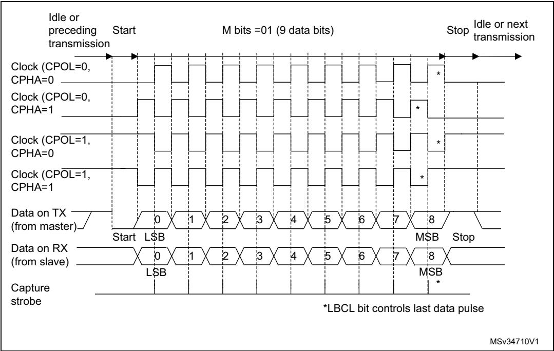
Figure 254. USART data clock timing diagram (M bits = 01)
