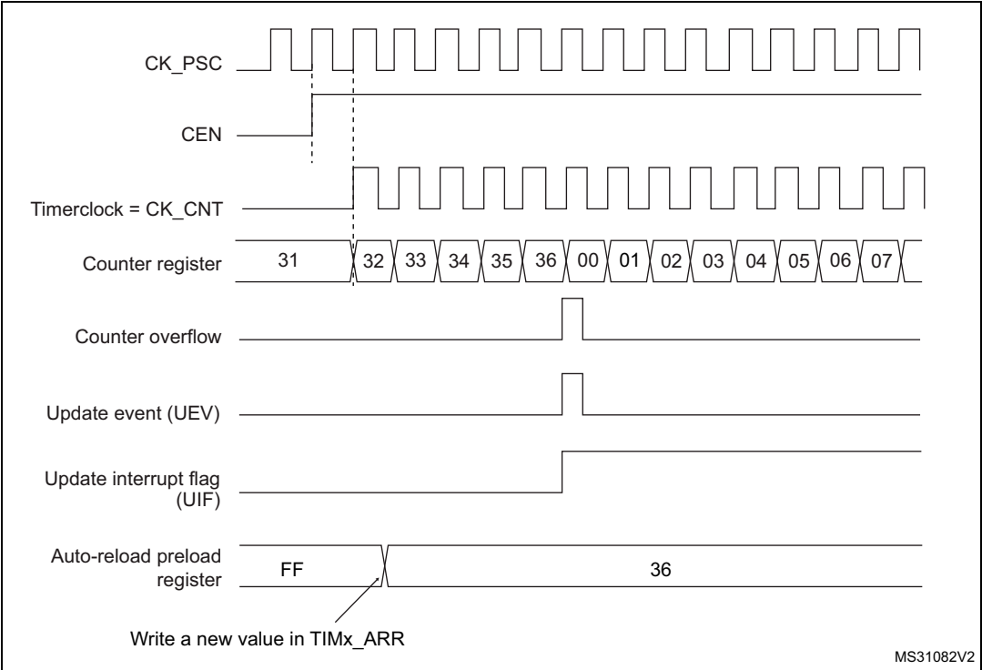
Figure 110. Counter timing diagram, Update event when ARPE=0 (TIMx_ARR not preloaded)
