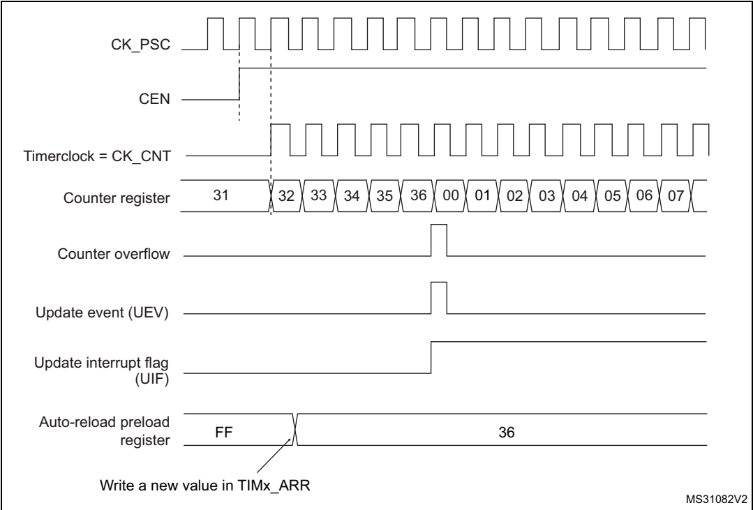
Figure 62. Counter timing diagram, update event when ARPE=0 (TIMx_ARR not preloaded)
