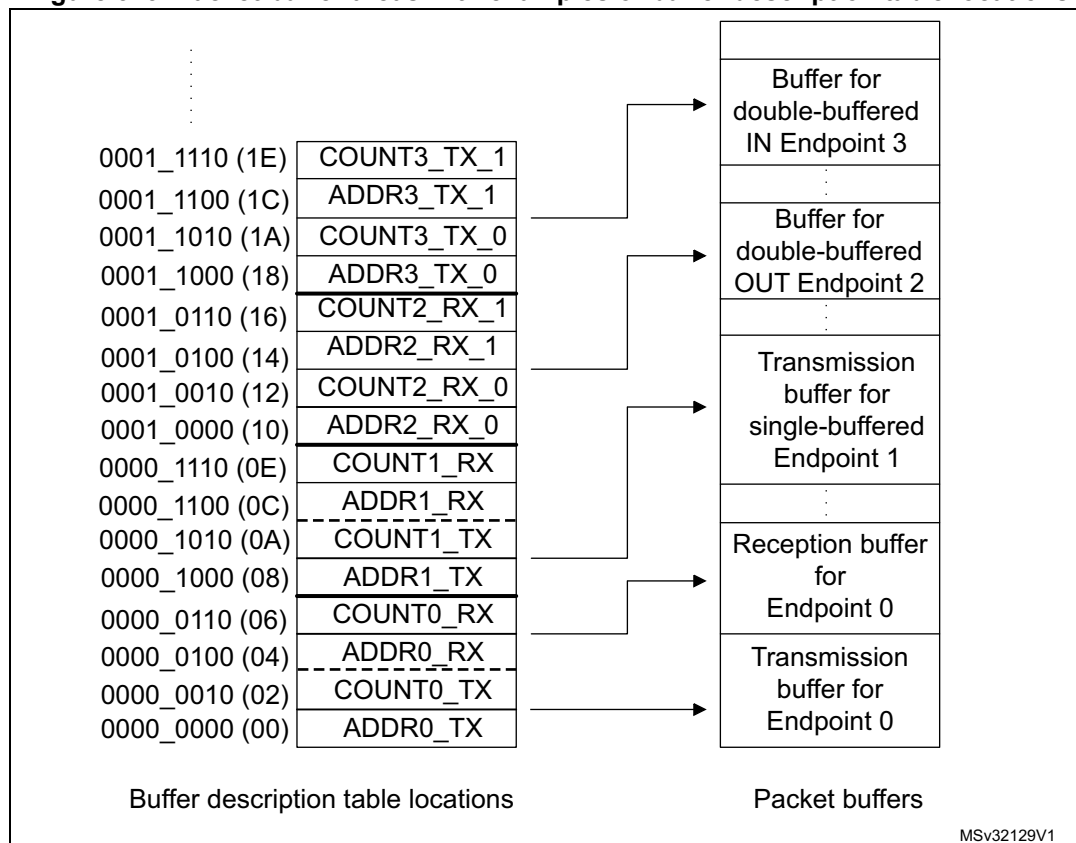
Figure 323. Packet buffer areas with examples of buffer description table locations
