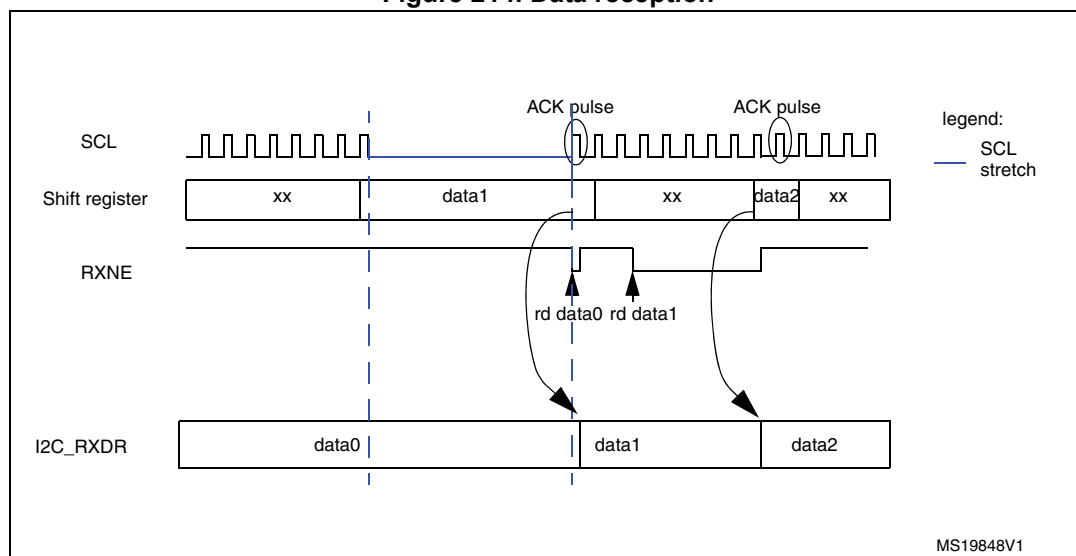
Figure 214. Data reception
