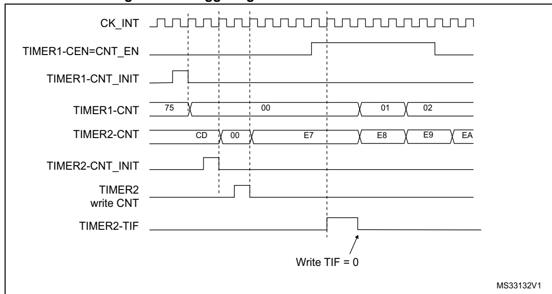
Figure 147. Triggering timer 2 with Enable of timer 1
