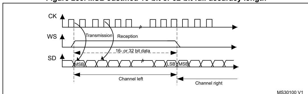
Figure 288. MSB Justified 16-bit or 32-bit full-accuracy length
