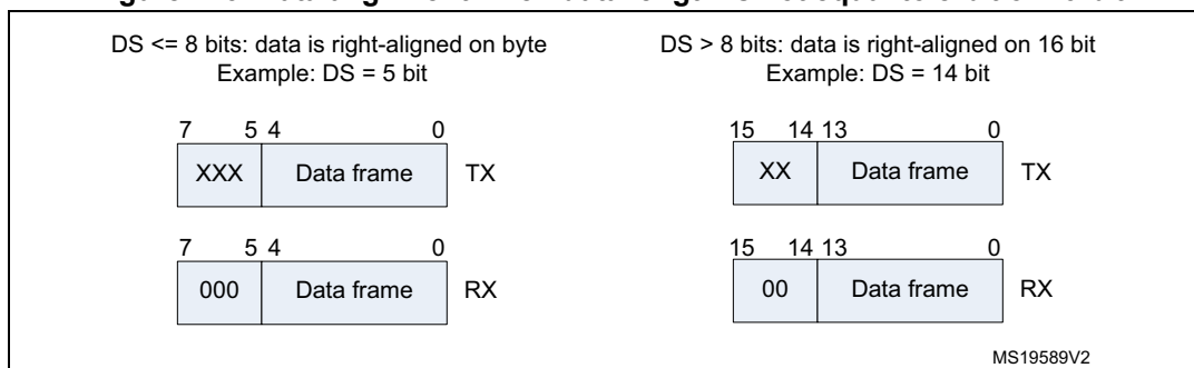
Figure 273. Data alignment when data length is not equal to 8-bit or 16-bit
