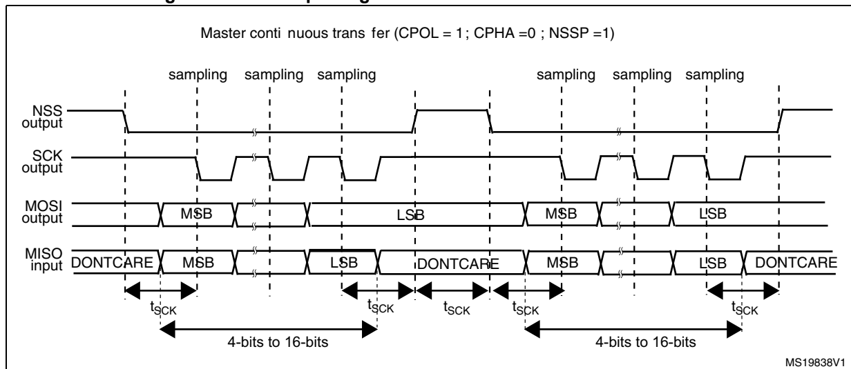
Figure 279. NSSP pulse generation in Motorola SPI master mode
