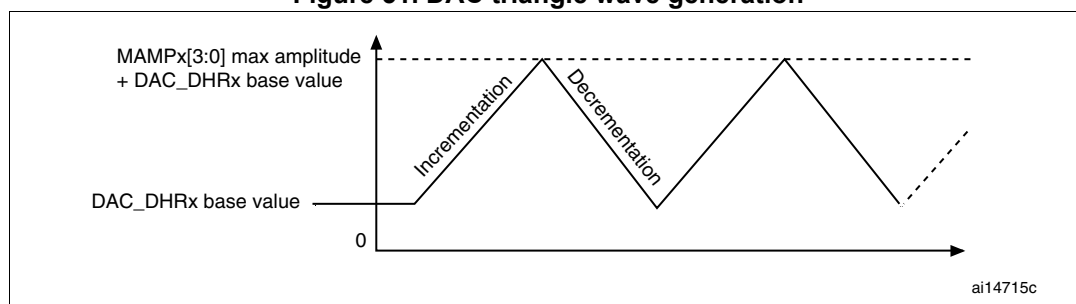
Figure 51. DAC triangle wave generation
