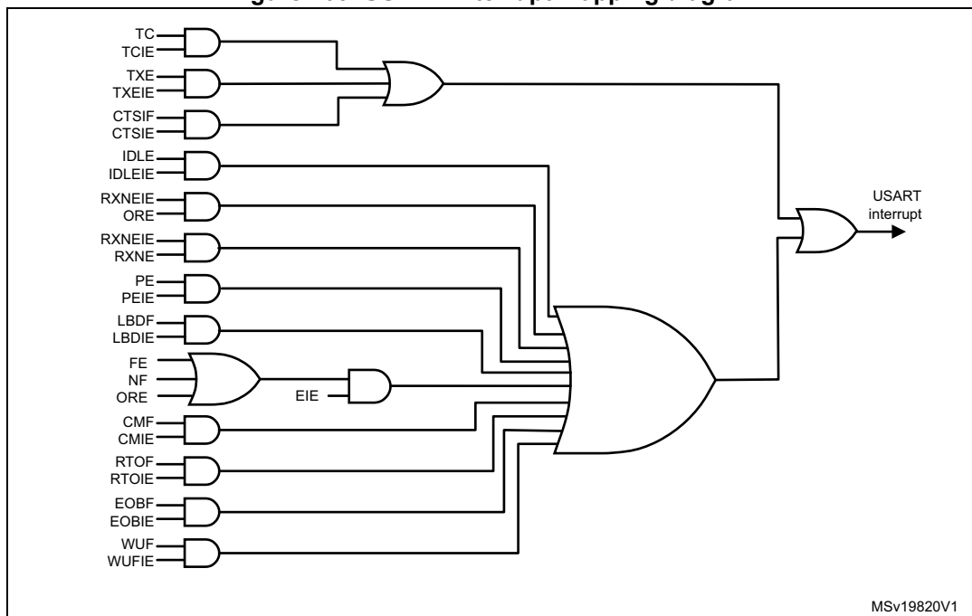
Figure 265. USART interrupt mapping diagram
