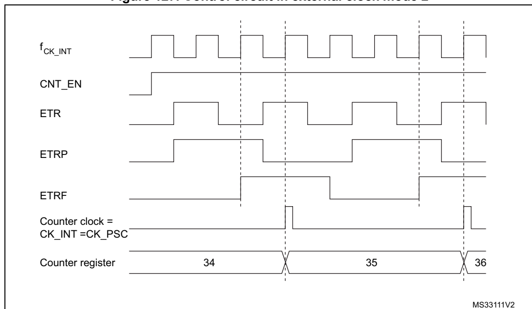
Figure 127. Control circuit in external clock mode 2
