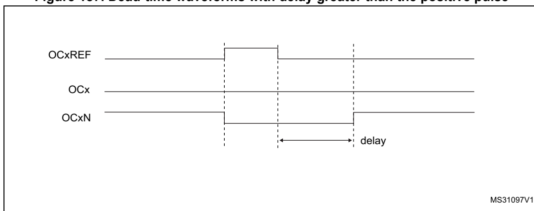
Figure 187. Dead-time waveforms with delay greater than the positive pulse
