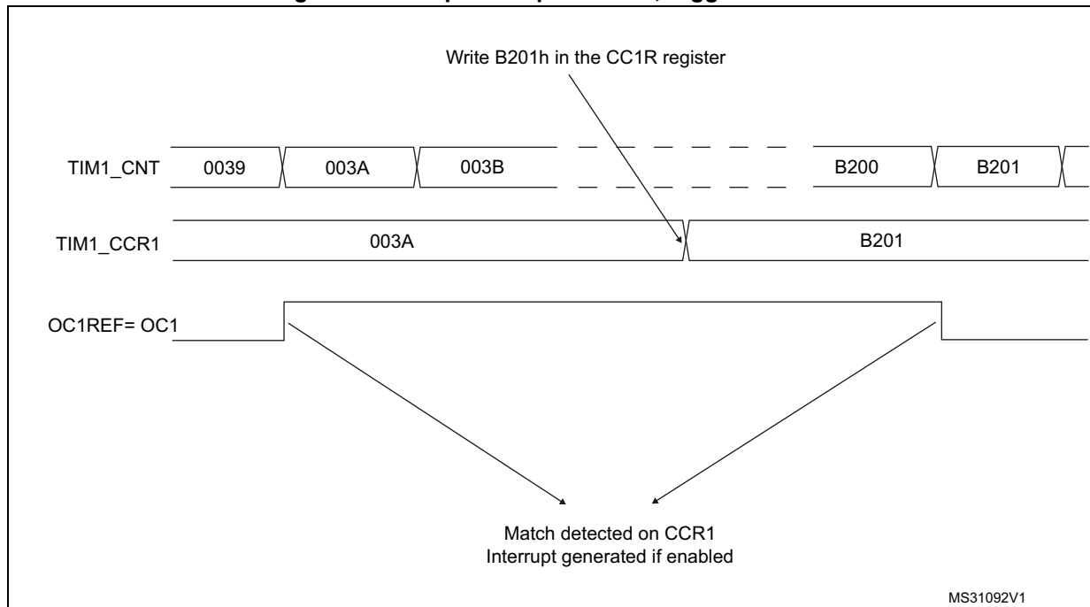
Figure 132. Output compare mode, toggle on OC1
