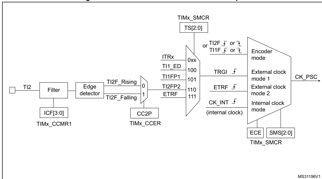
Figure 124. TI2 external clock connection example
