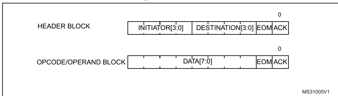
Figure 326. Blocks
