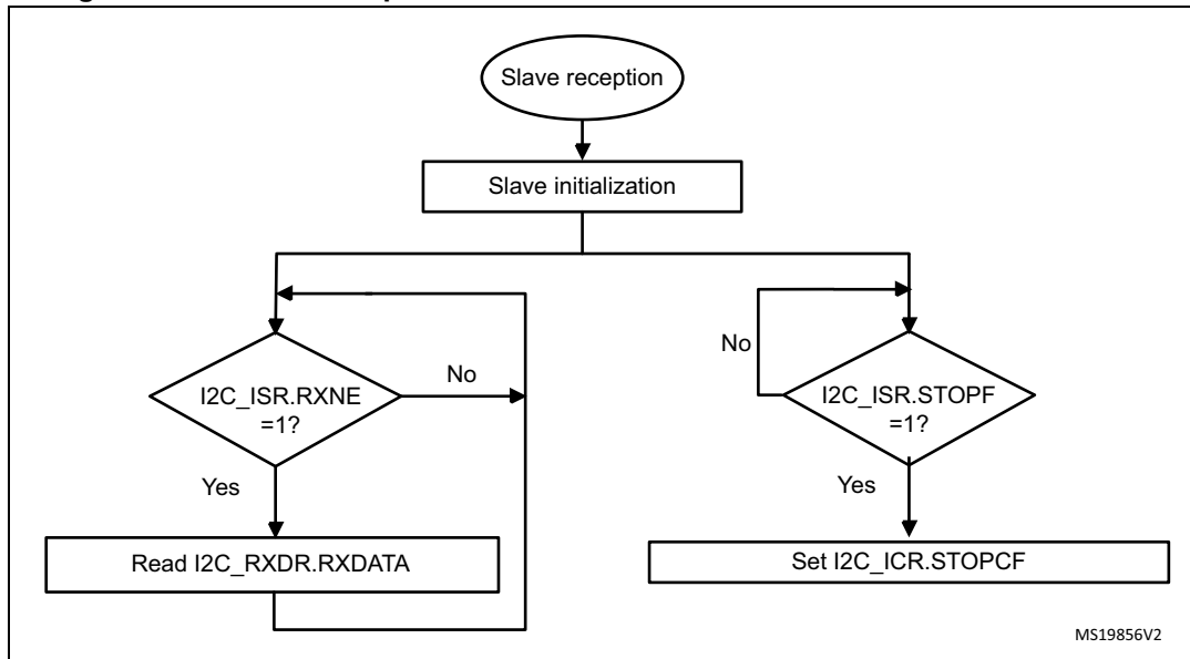
Figure 221. Transfer sequence flowchart for slave receiver with NOSTRETCH=1
