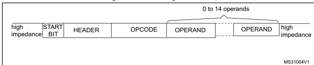
Figure 325. Message structure
