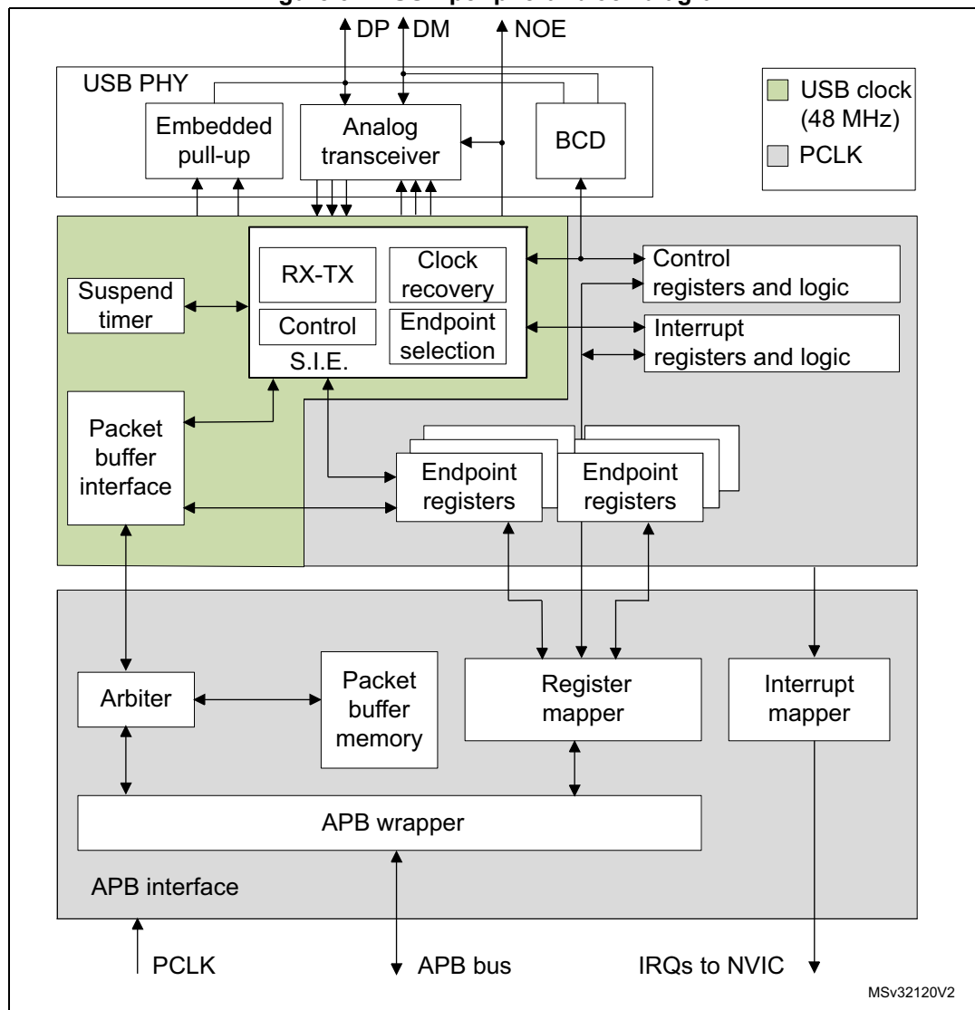
Figure 322. USB peripheral block diagram
