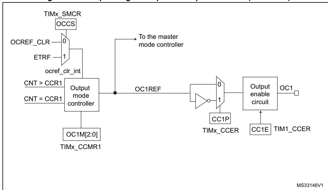
Figure 130. Output stage of capture/compare channel (channel 1)
