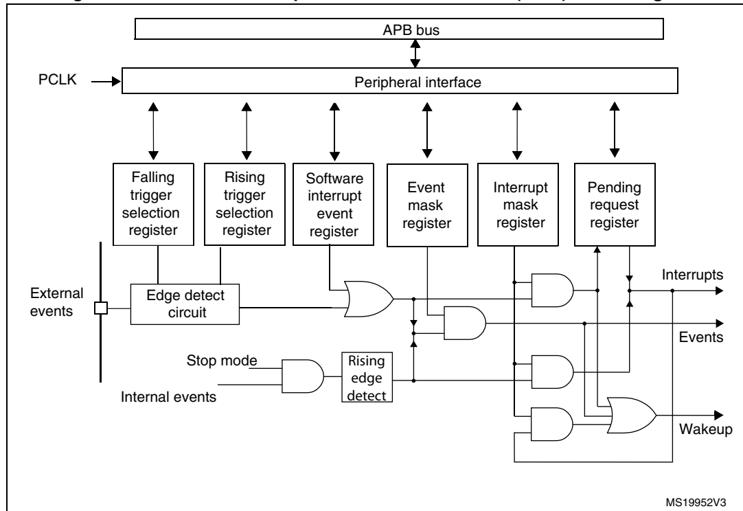
Figure 24. Extended interrupts and events controller (EXTI) block diagram
