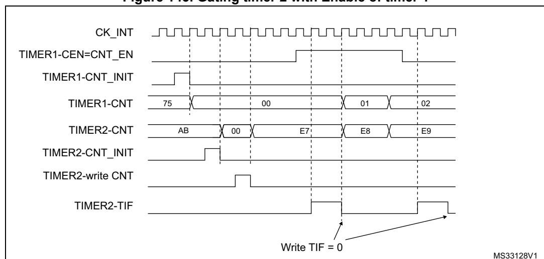
Figure 145. Gating timer 2 with Enable of timer 1
