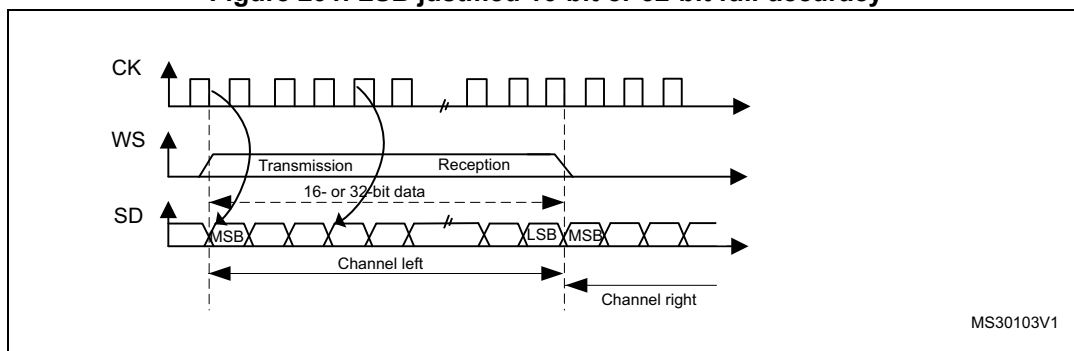
Figure 291. LSB justified 16-bit or 32-bit full-accuracy
