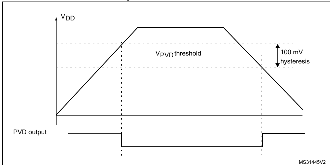
Figure 9. PVD thresholds
