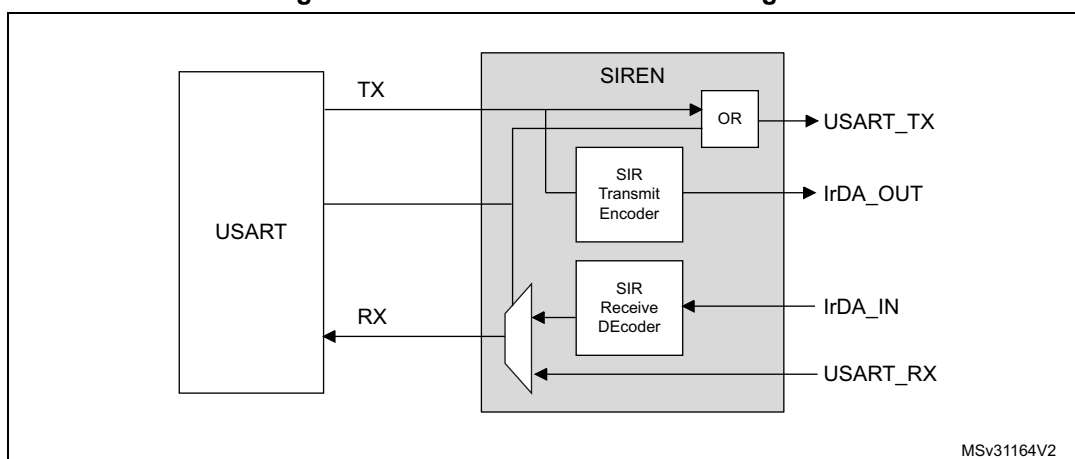
Figure 258. IrDA SIR ENDEC- block diagram
