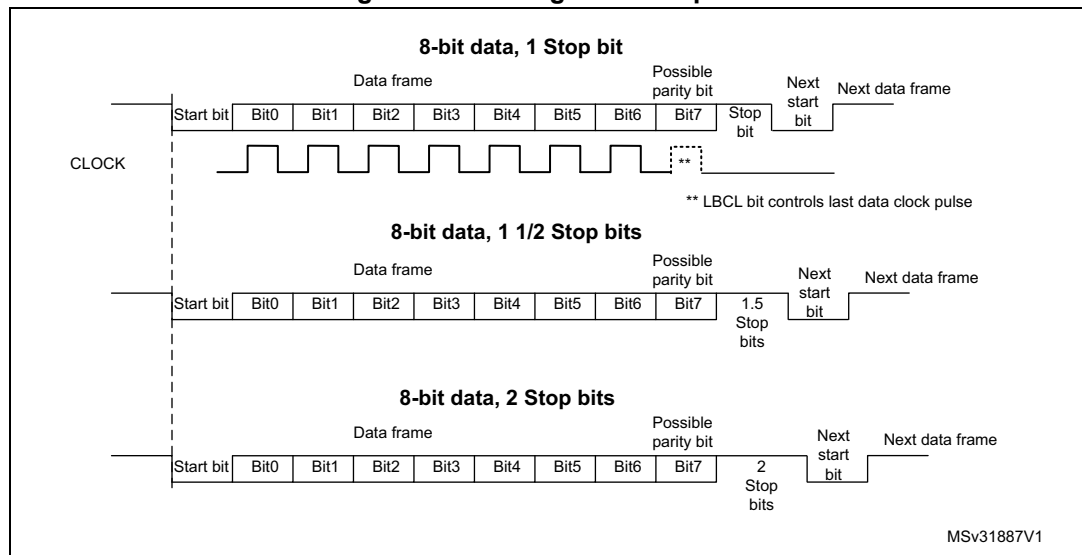
Figure 243. Configurable stop bits
