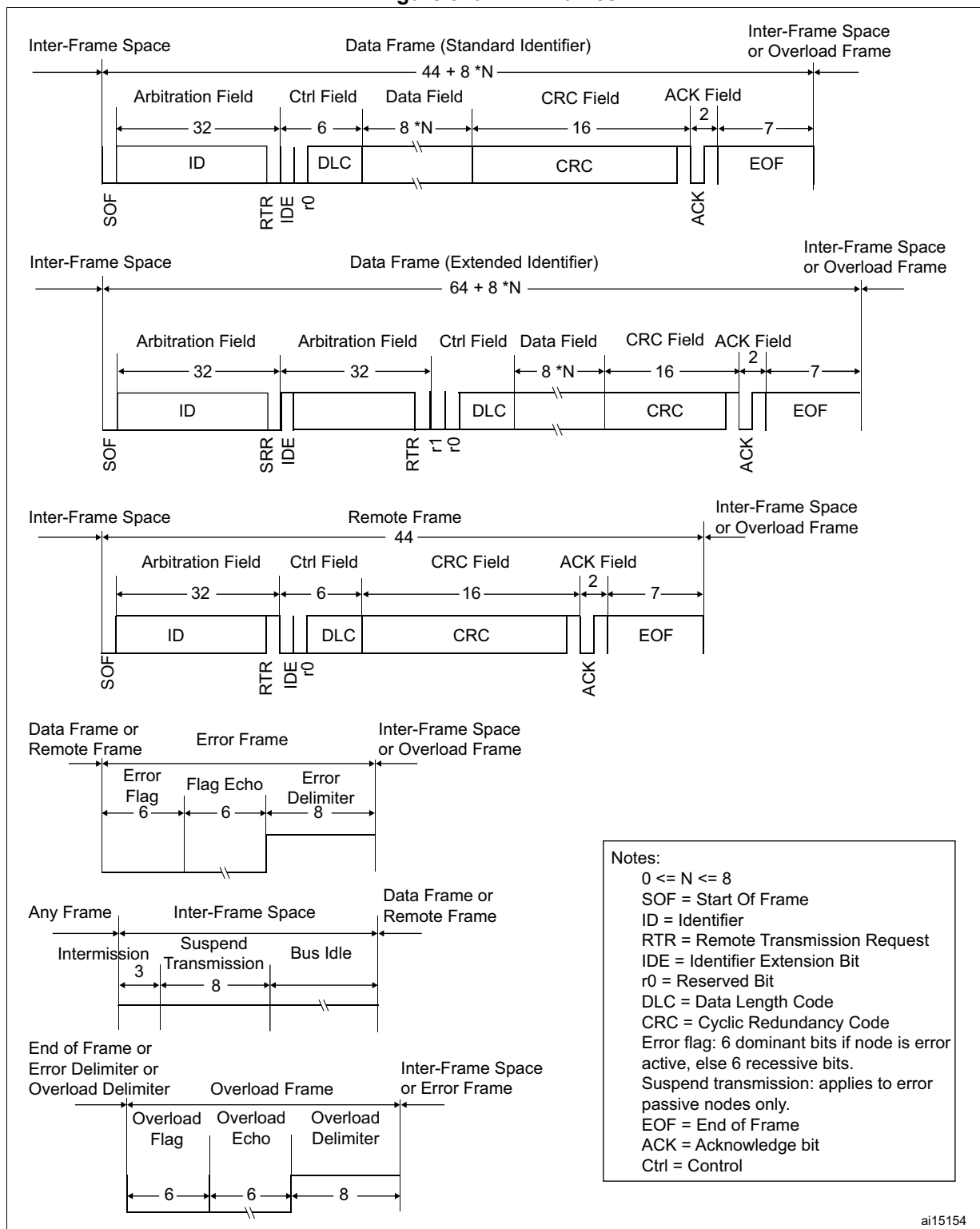
Figure 319. CAN frames
