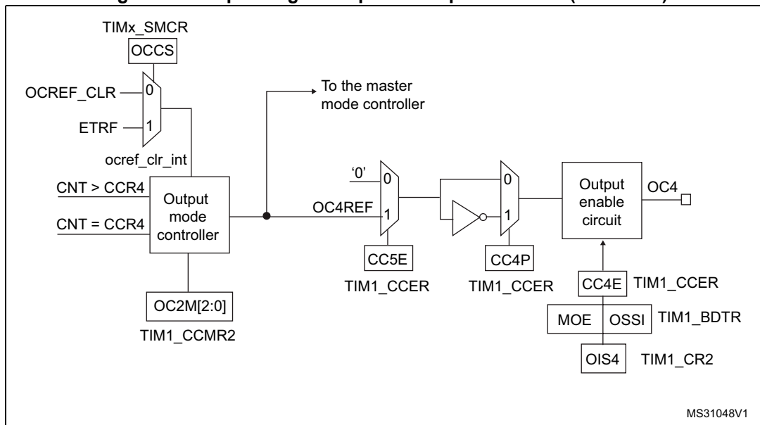
Figure 84. Output stage of capture/compare channel (channel 4)
