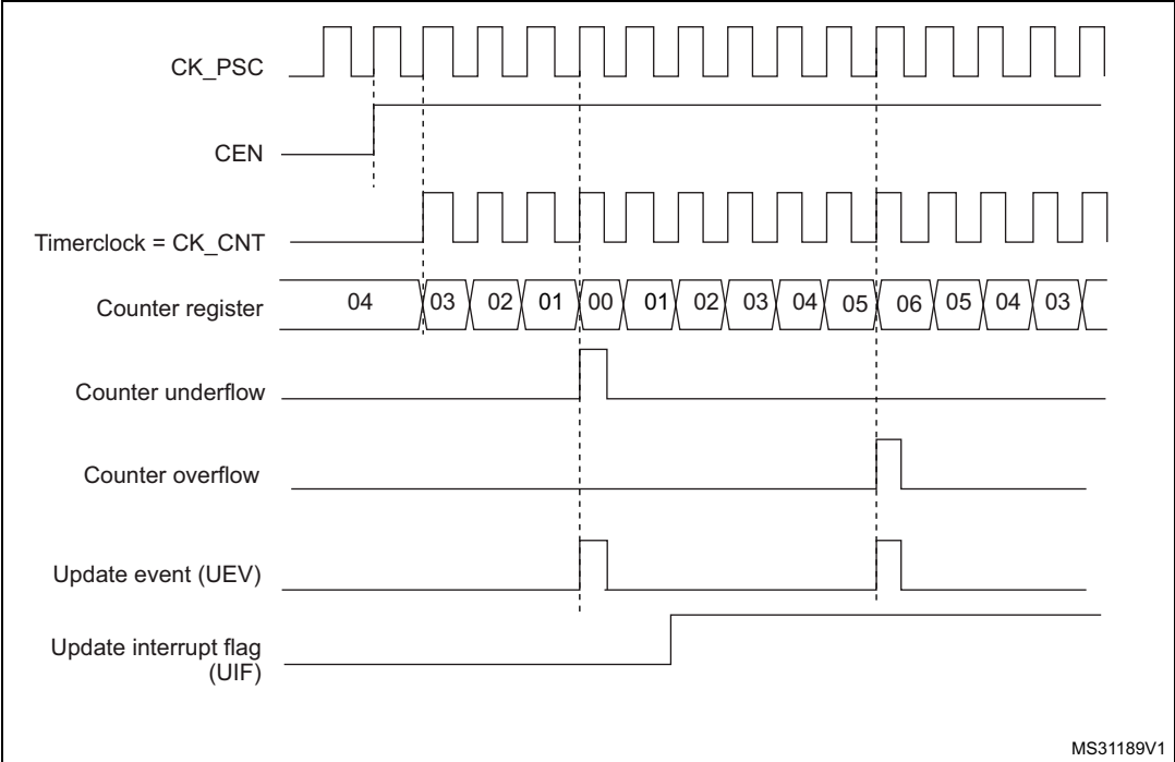
Figure 117. Counter timing diagram, internal clock divided by 1, TIMx_ARR=0x6
