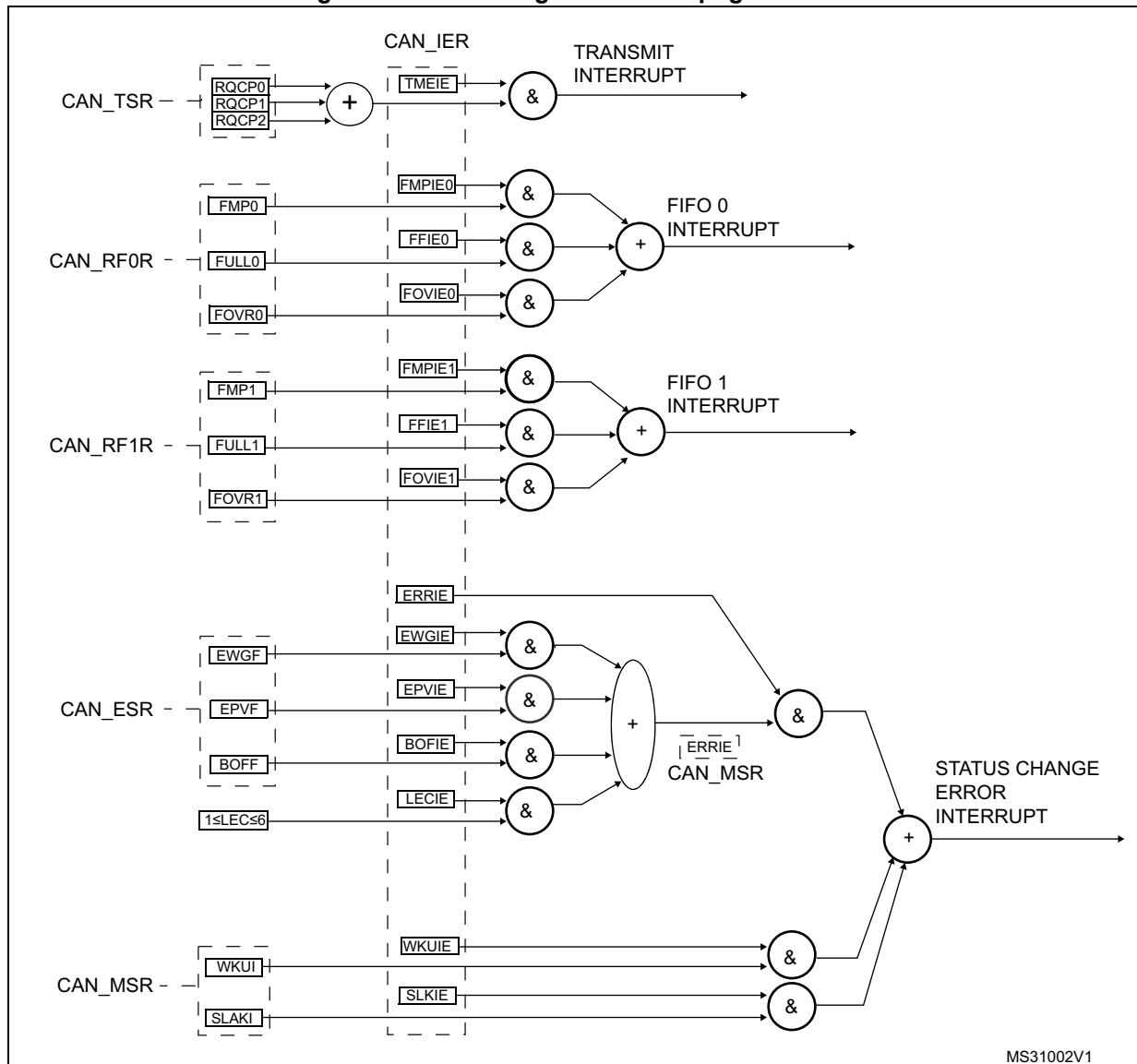
Figure 320. Event flags and interrupt generation
