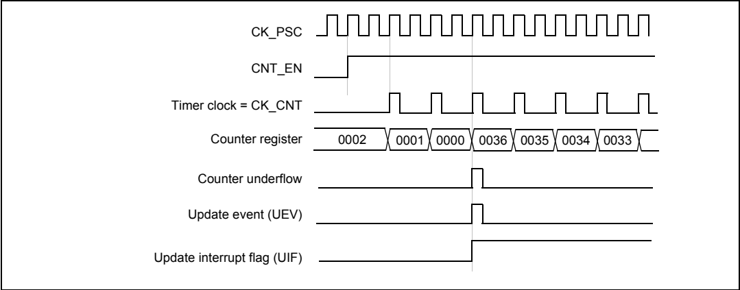
Figure 65. Counter timing diagram, internal clock divided by 2
