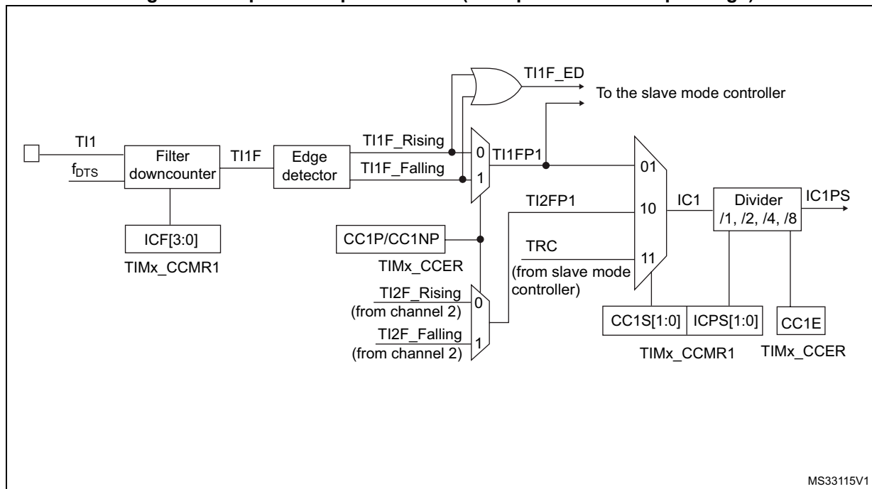
Figure 81. Capture/compare channel (example: channel 1 input stage)
