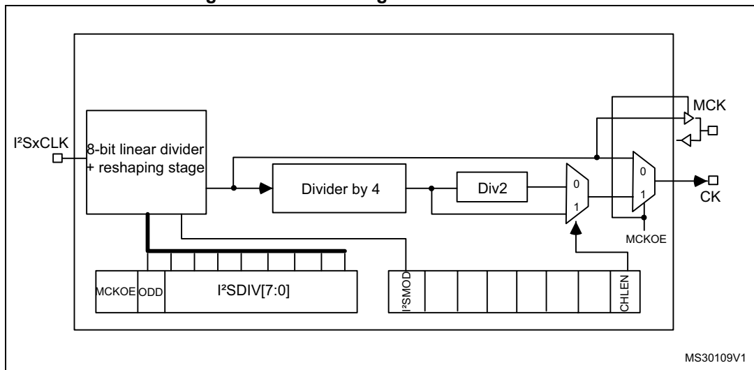
Figure 301. I 2 S clock generator architecture
