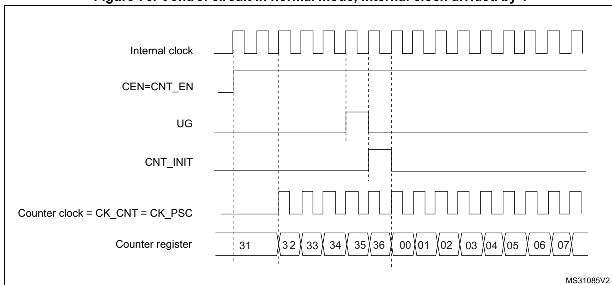
Figure 76. Control circuit in normal mode, internal clock divided by 1
