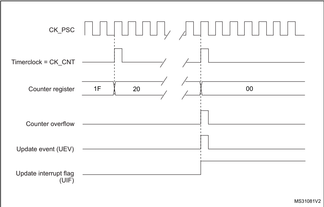
Figure 199. Counter timing diagram, internal clock divided by N
