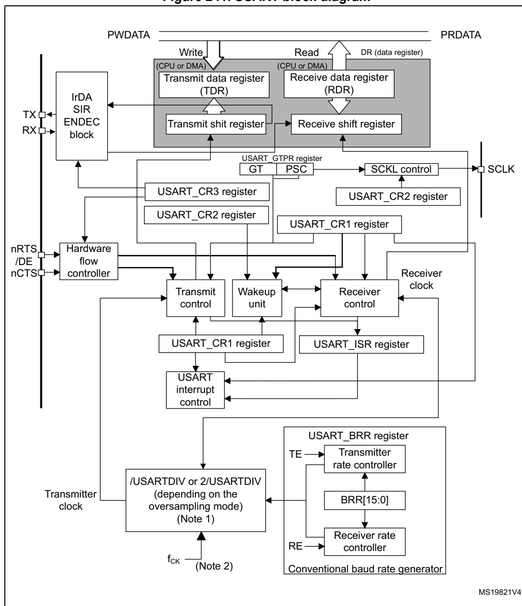
Figure 241. USART block diagram
