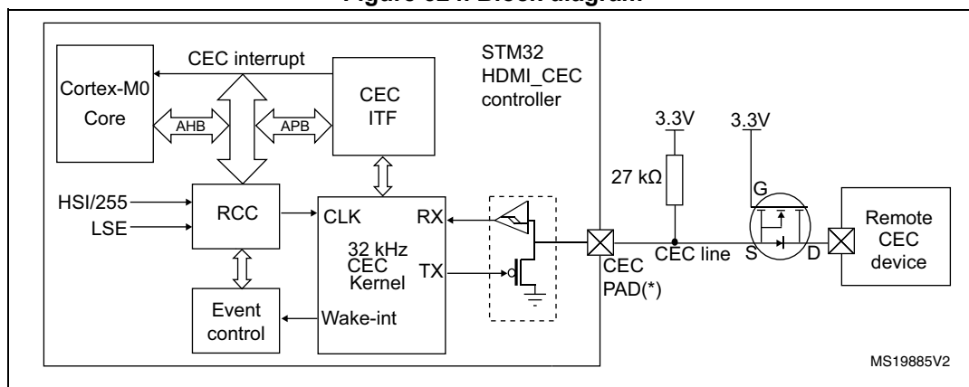
Figure 324. Block diagram
