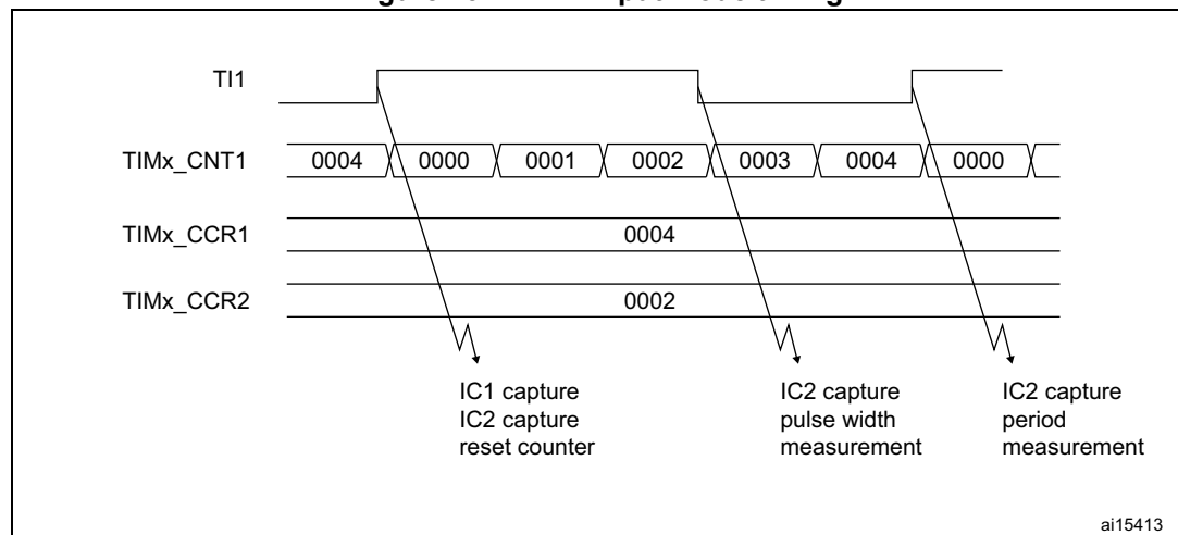
Figure 131. PWM input mode timing
