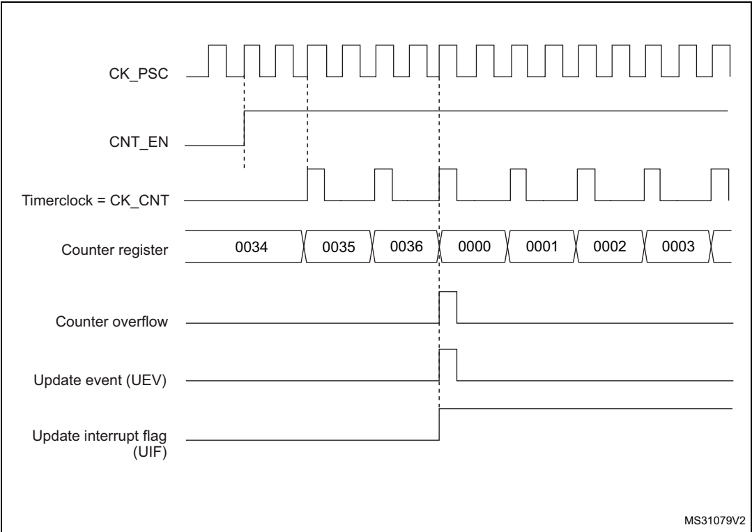
Figure 197. Counter timing diagram, internal clock divided by 2
